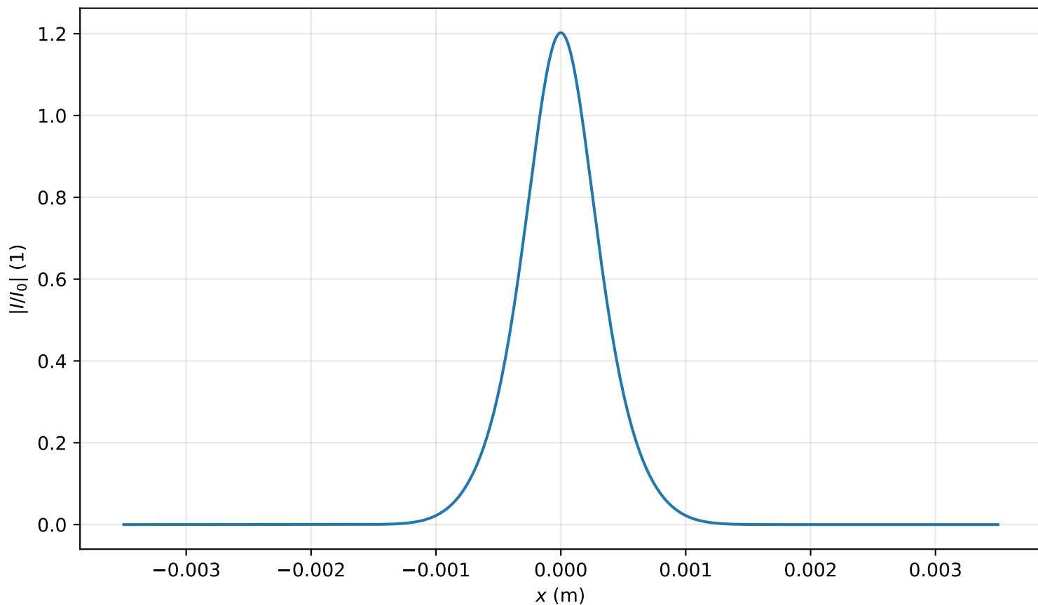
Intensity profile I(x, y = 0, z = 0.716m)/I_0 , P_{in}=0.8P_{cr} , artificial time
